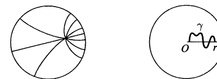
hyperbolic geodesics
